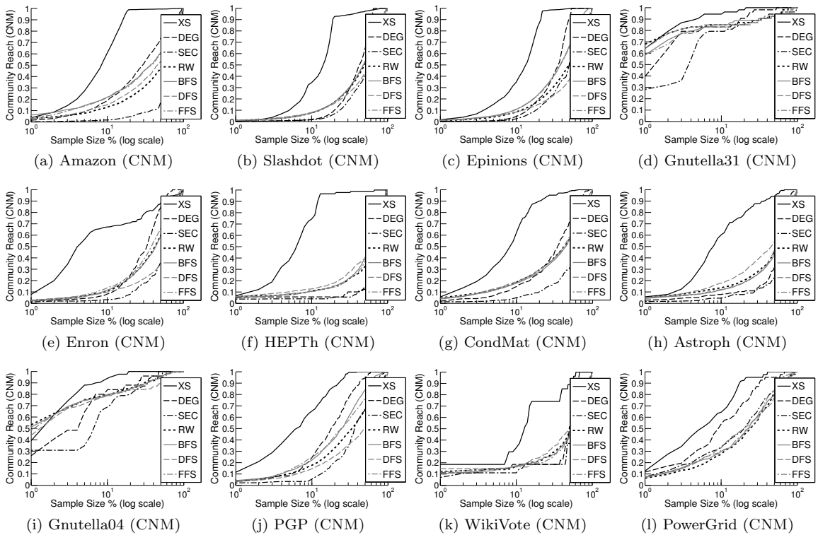
Figure 7: Full results for CNM.
