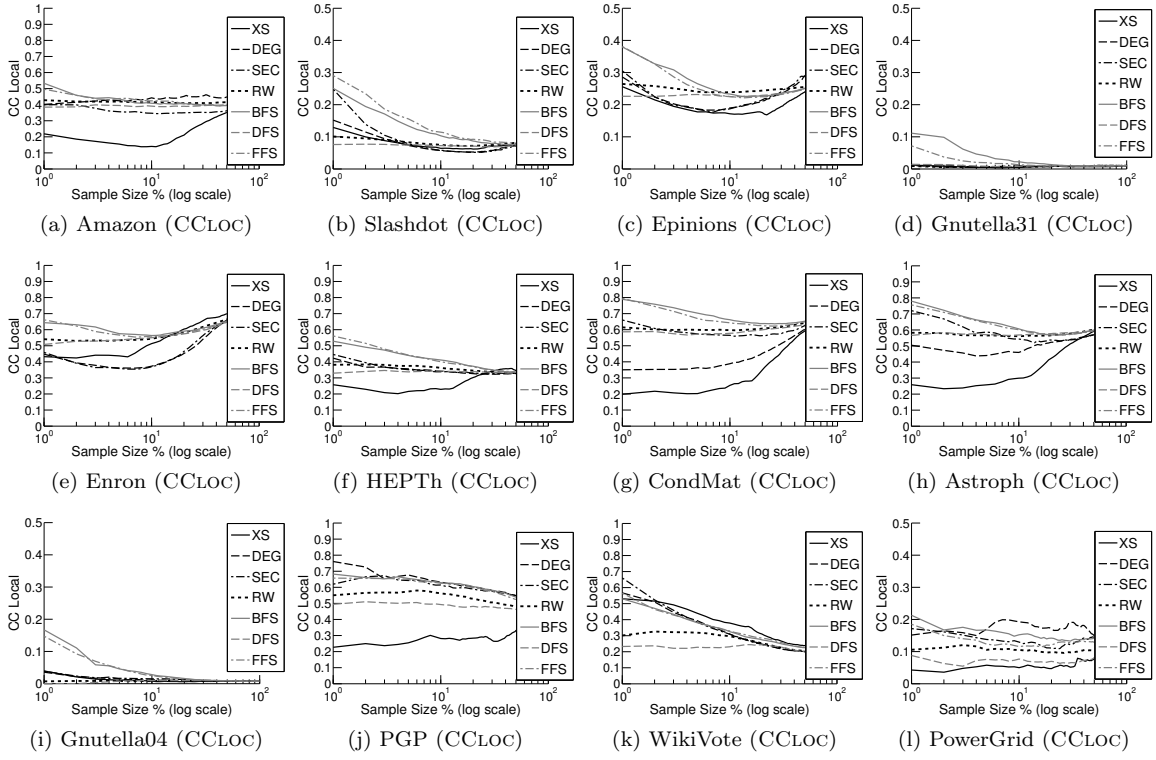
Figure 4: Full results for CCLOC.
