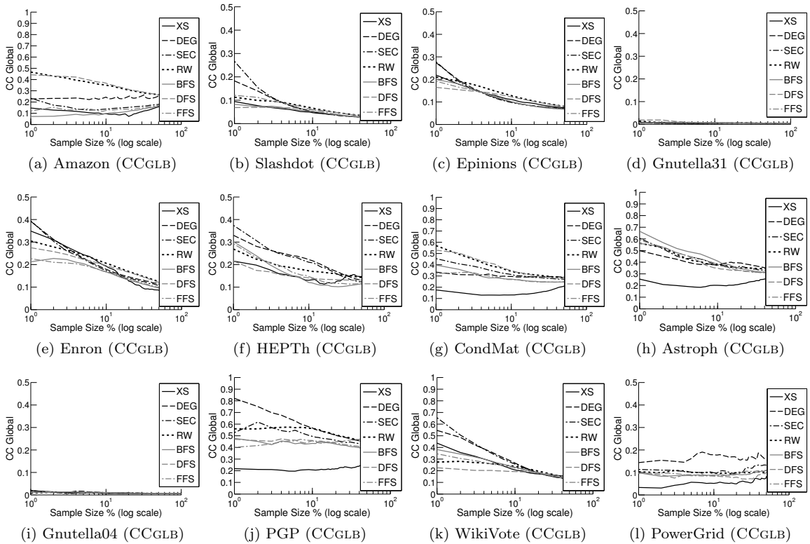
Figure 5: Full results for CCGLB.
