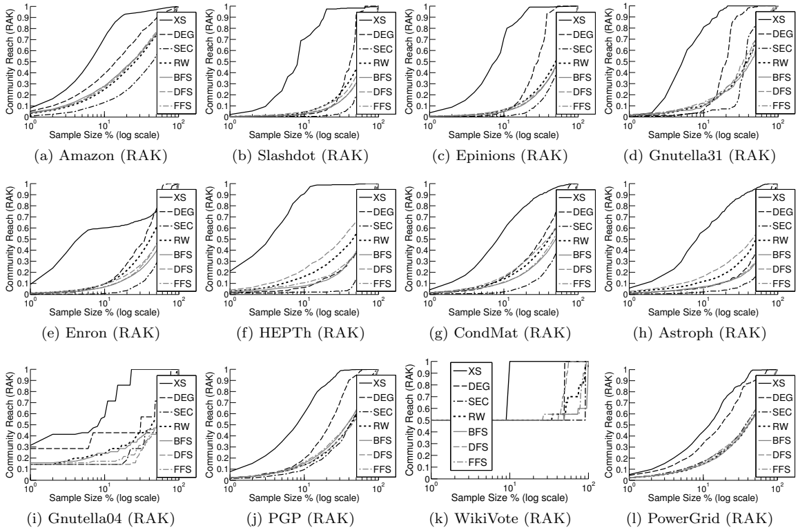
Figure 6: Full results for RAK.
