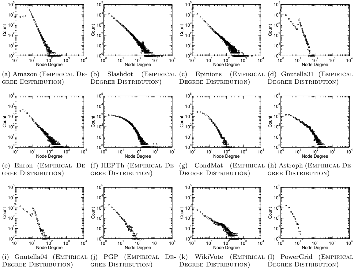
Figure 3: Full results for EMPIRICAL DEGREE DISTRIBUTIONS.
