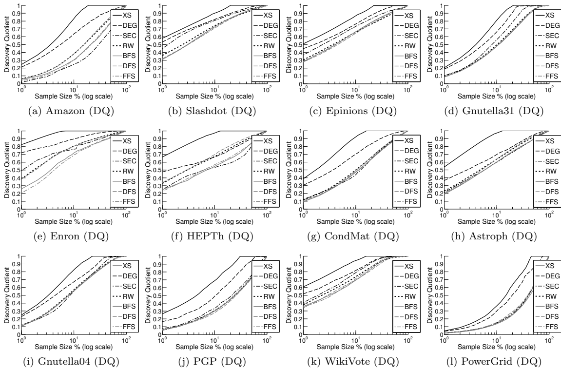
Figure 8: Full results for DQ.
