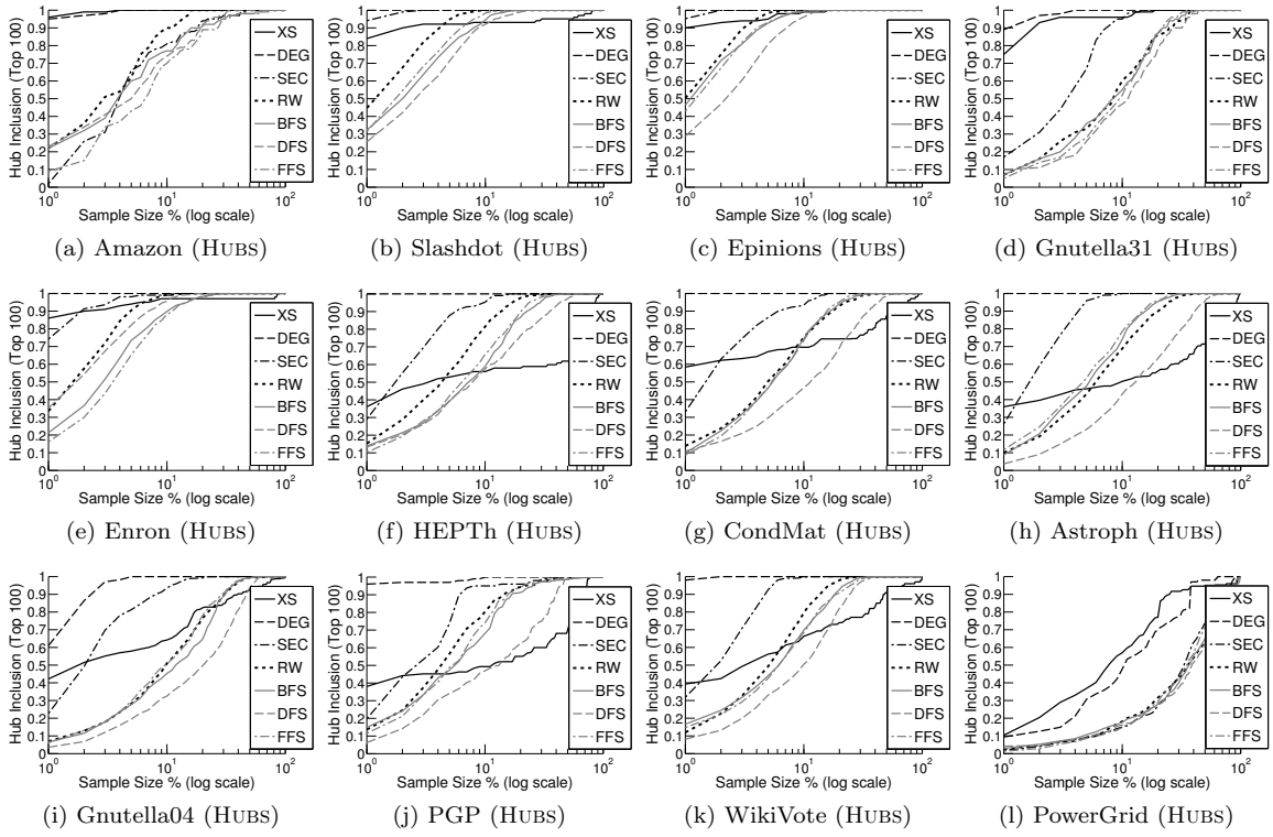
Figure 2: Full results for HUBS.
